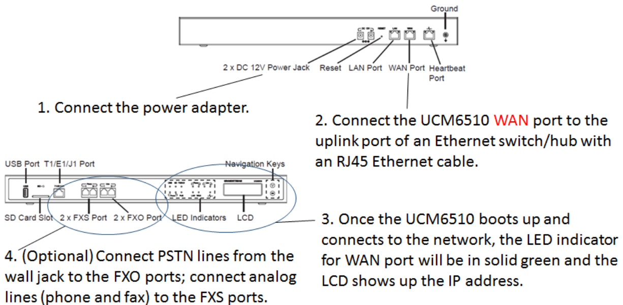
Figure 2: Connecting UCM6510
